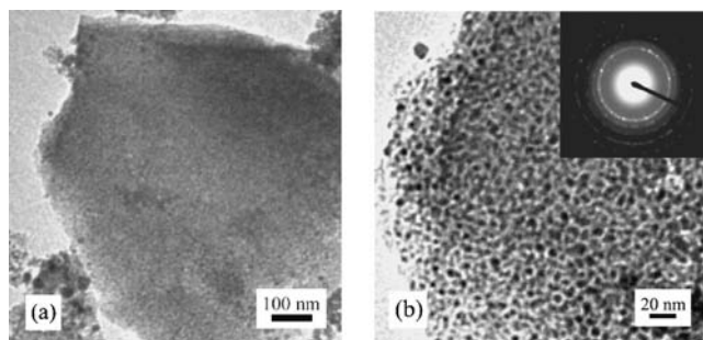
Figure 2. TEM images of the sample calcined in \text{N}_2 : (a) low-magnification image; (b) high-magnification image and the SAED patterns (inset).
