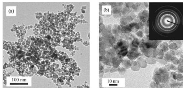
Figure 1. TEM images of the NiO sample: (a) low-magnification image; (b) high-magnification image and the corresponding SAED patterns (inset).
